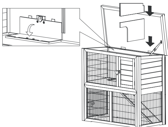
Step 5. Put down Lower & Upper Partitions .
