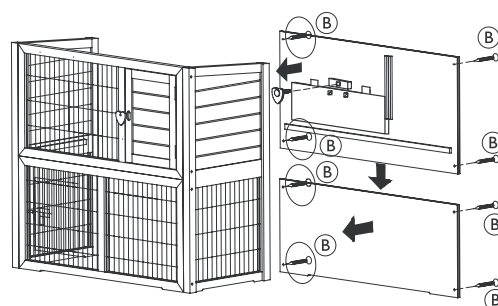
Step 2. Install the Lower & Upper Back Panels.
