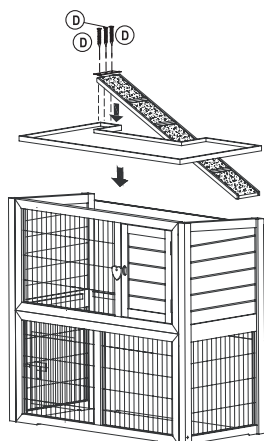
Step 3. Put down Mid-Floor & Ladder , Secure Ladder on Mid-Floor .
